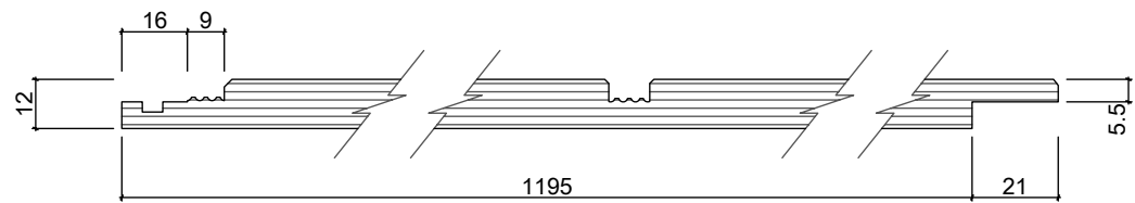
Groove Profile
