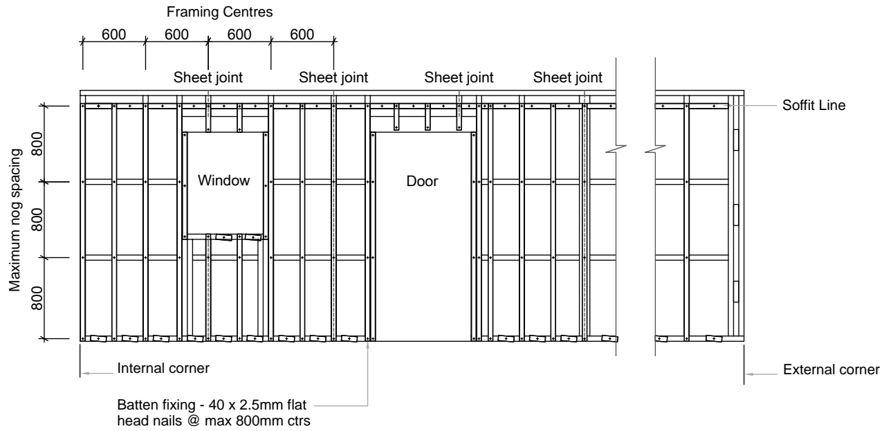
SC002 Shadowclad Framing Layout with Cavity Battens
