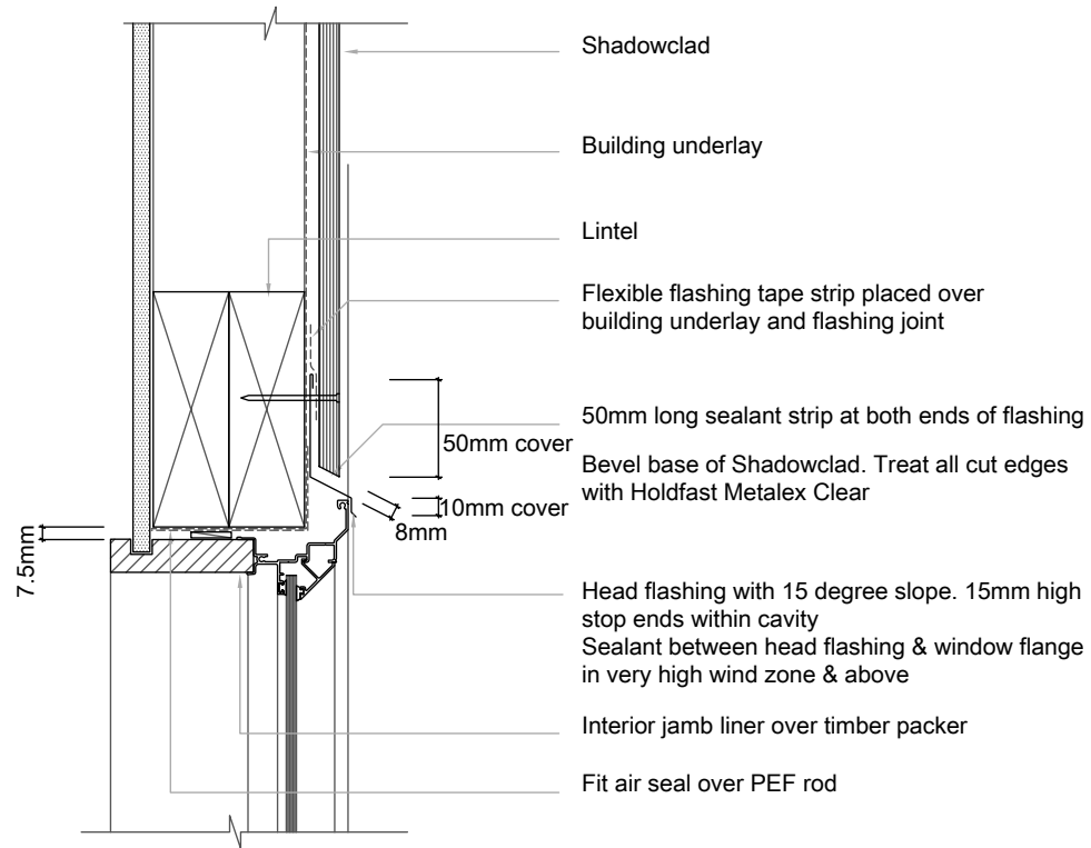
SC027 Shadowclad Window Head (Direct)
