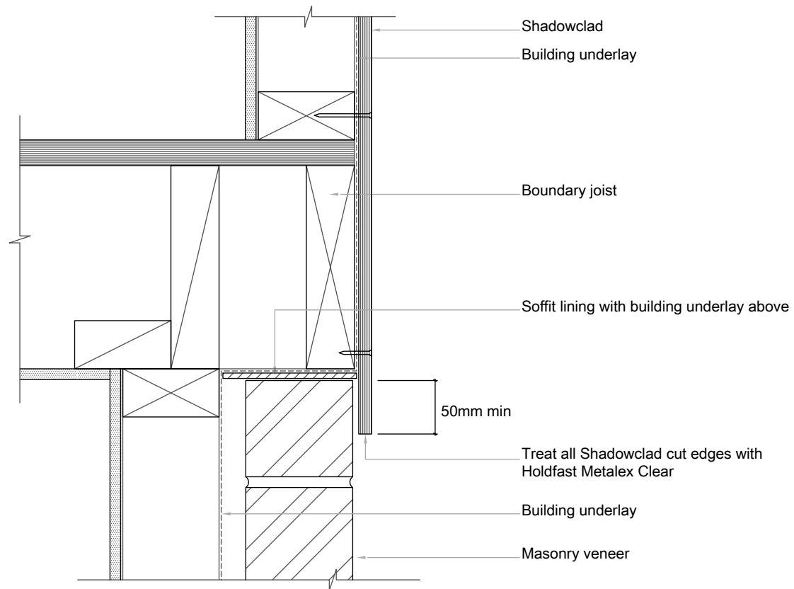
Vertical section
