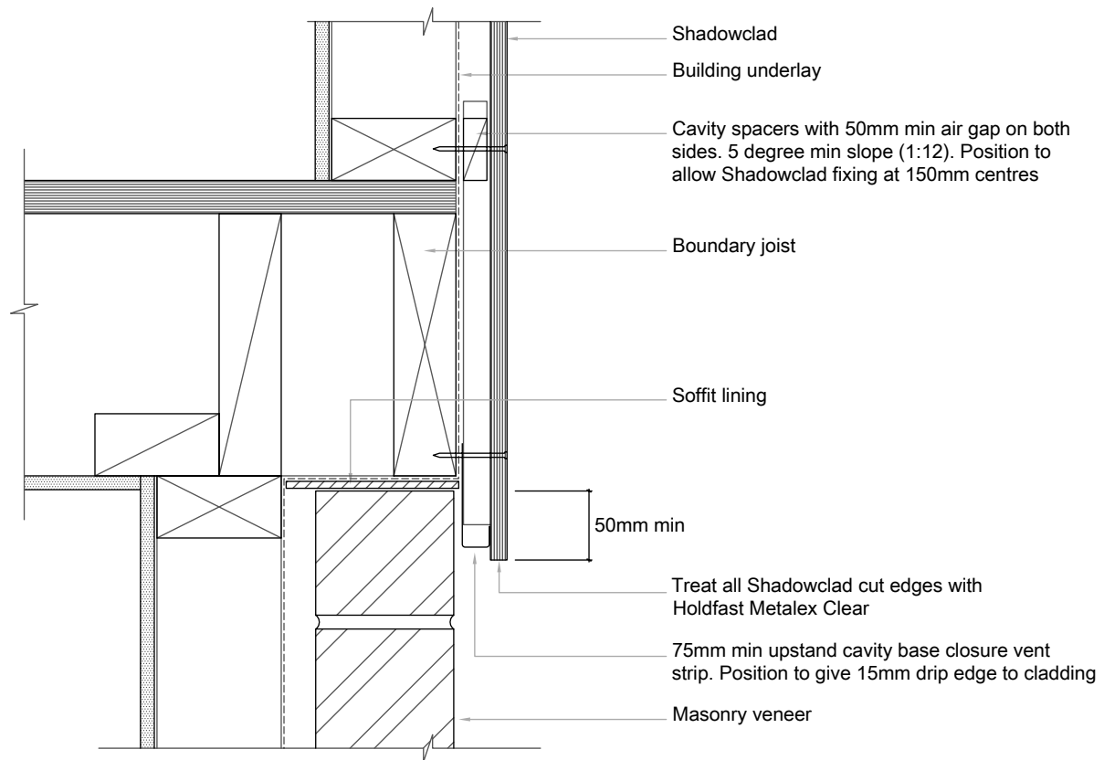
Vertical section
