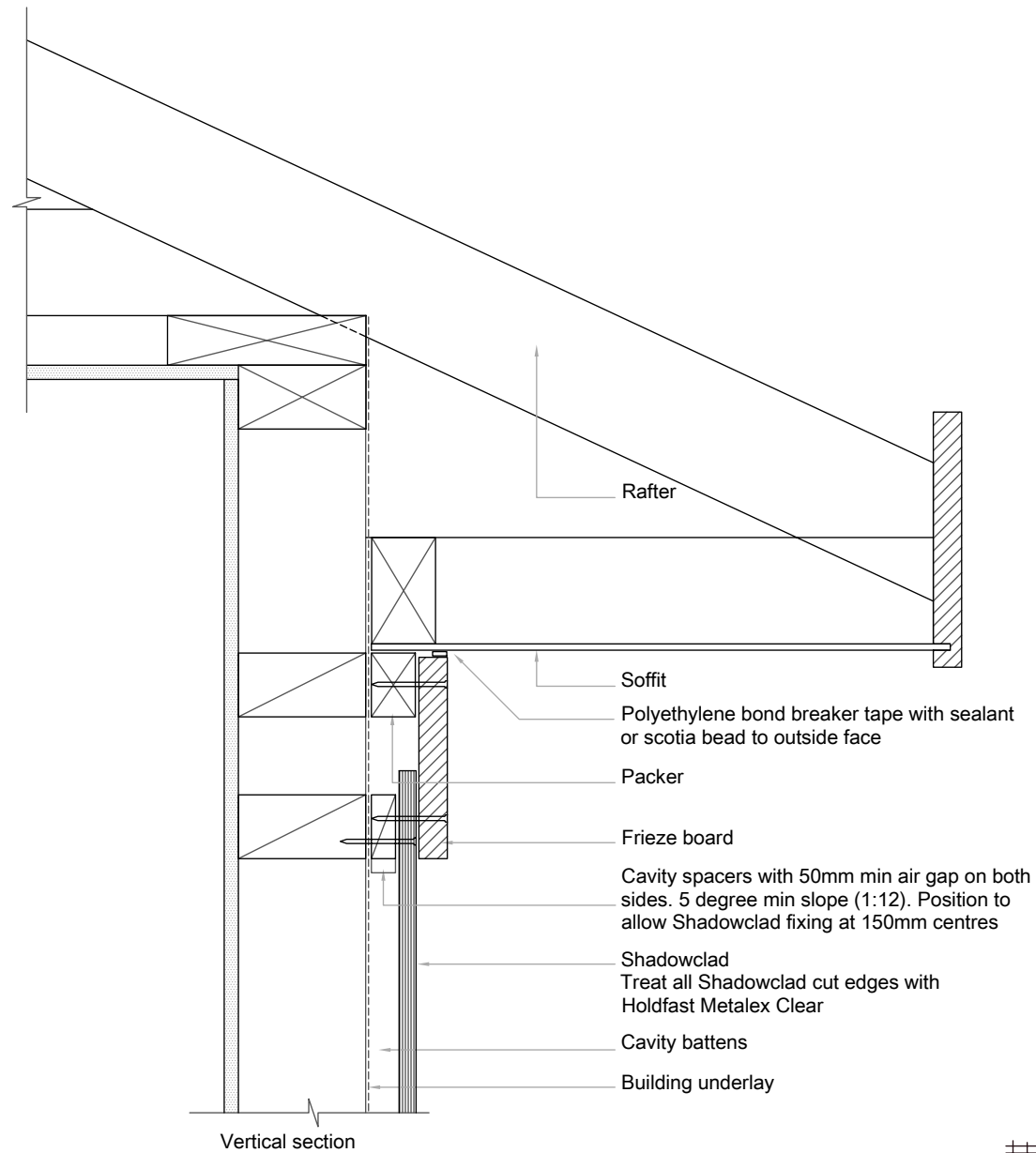
SC038 Shadowclad Soffit Alternative Detail (Cavity)
