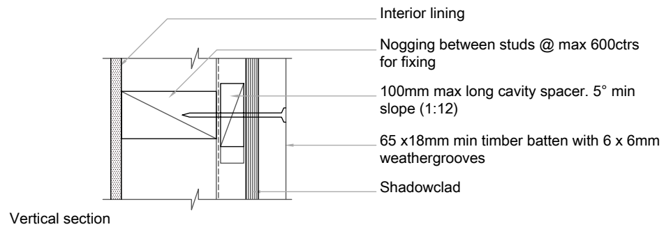
SC012 Shadowclad Vertical Joint with Optional Cover Batten (Cavity)
