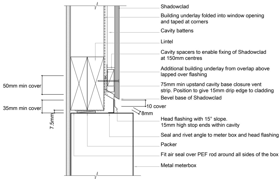
SC034A Shadowclad Meterbox Side Profile (Cavity)
