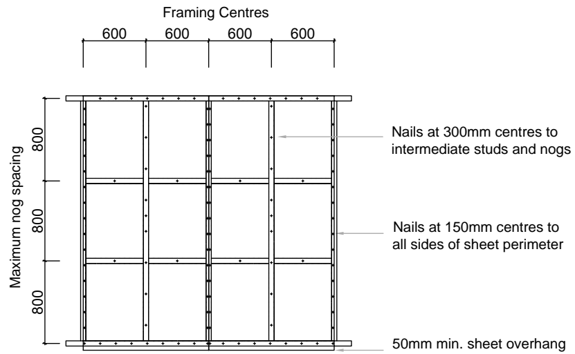
SC003 Shadowclad Fastener Layout
